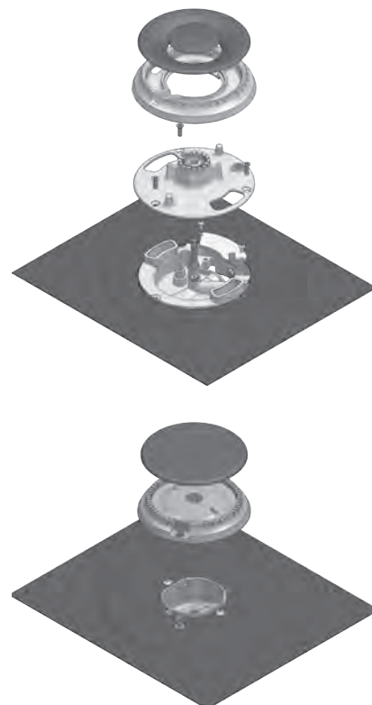
EXPLODED VIEW OF BURNER
