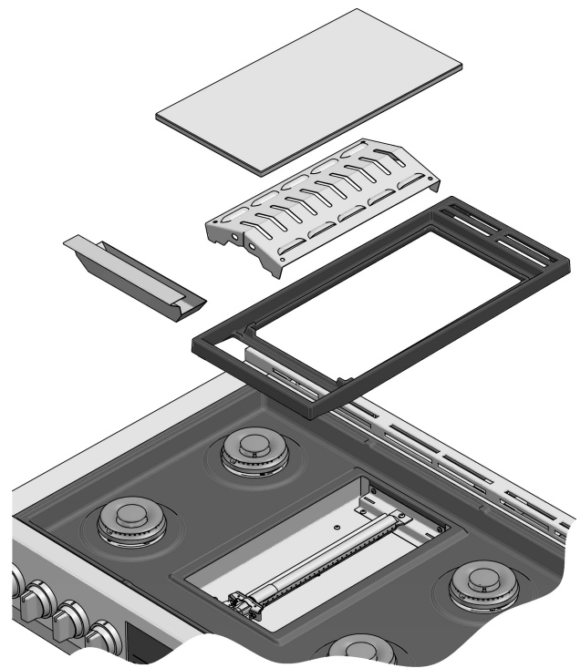
EXPLODED VIEW OF BURNER GRIDDLE
